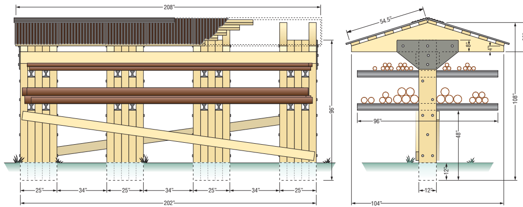
Engine Boiler Flue Storage Rack drawn by G. M. McKenzie scale: 3/16" = 1'
