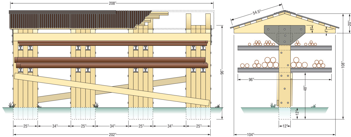
Engine Boiler Flue Storage Rack drawn by G. M. McKenzie scale: 1/4" = 1'
